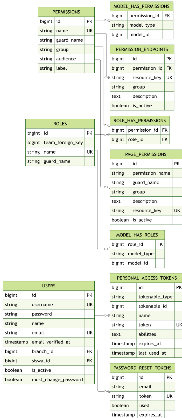
Gambar 3.5. Diagram Relasi Tabel Modul RBAC Dinamis &amp; Auth
