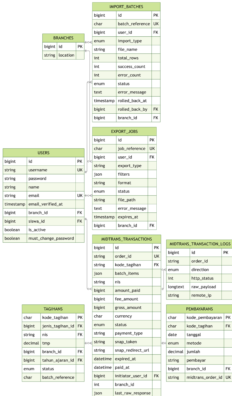
Gambar 3.8. Diagram Relasi Tabel Modul Import/Export &amp; Midtrans
