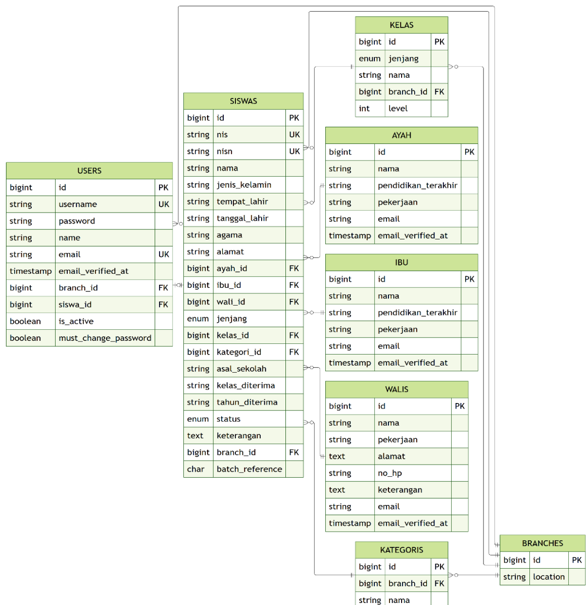
Gambar 3.3. Diagram Relasi Tabel Data Master
